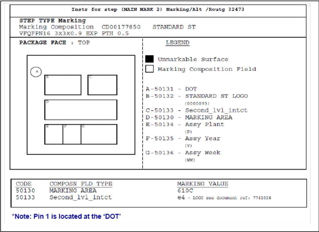
Figure 17. Marking specifications
