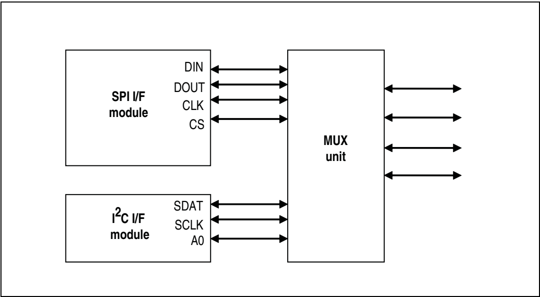
Figure 3. STMPE610 interface
