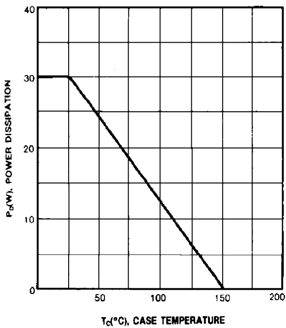
POWER DERATING
