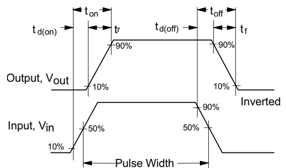
Figure 12. Switching Waveforms.
