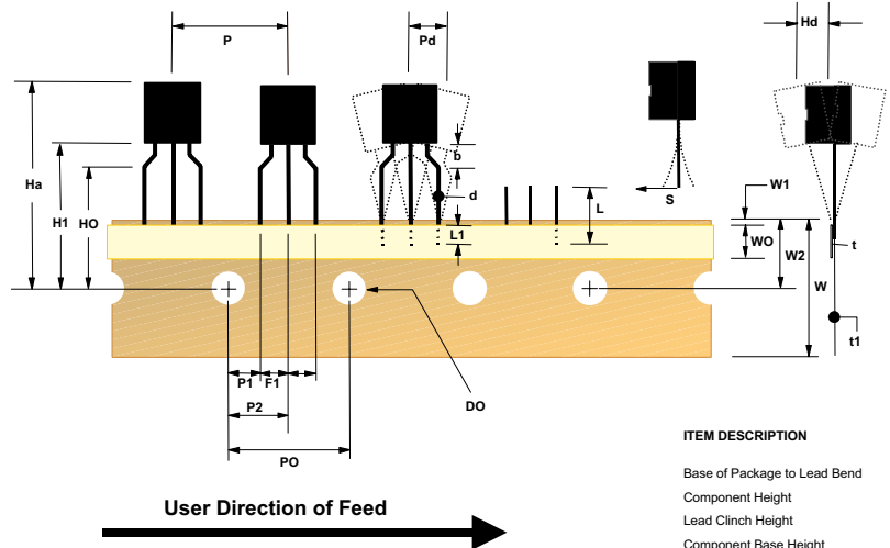
TO-92 Tape and Reel Taping Dimension Configuration: Figure 4.0
