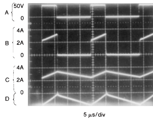
Switching Waveforms
