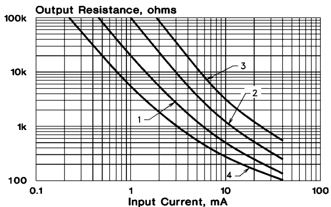
Output Resistance vs. Input Current
