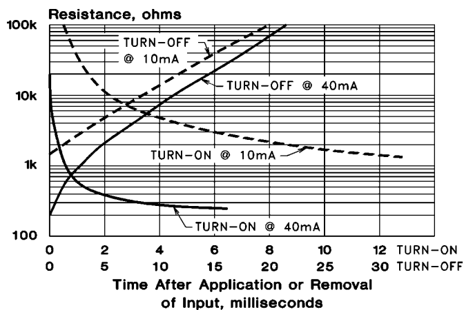
Response Time
