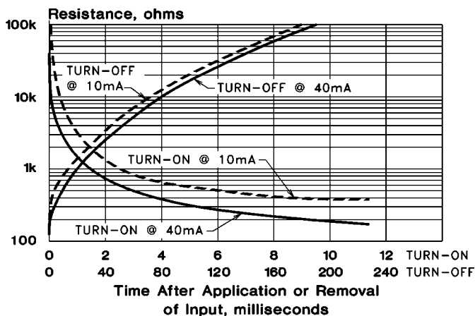
Response Time
