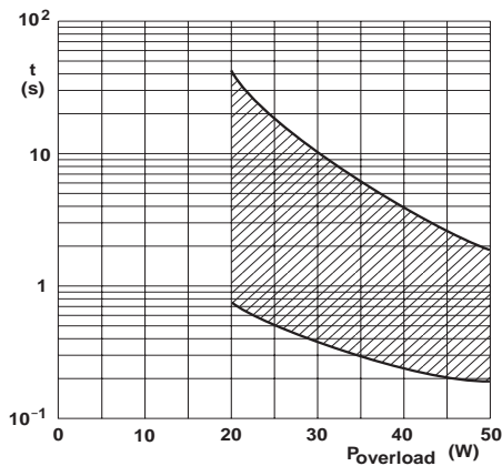
PR01 Time to interruption as a function of overload power for range: 1 R \leq R_n \leq 15 R .
