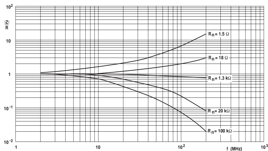
PR03 Impedance as a function of applied frequency.
