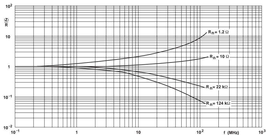
PR02 Impedance as a function of applied frequency.
