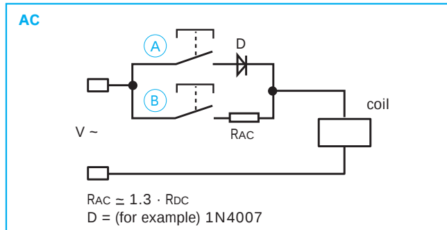
DRIVING CIRCUIT (AC · DC)
