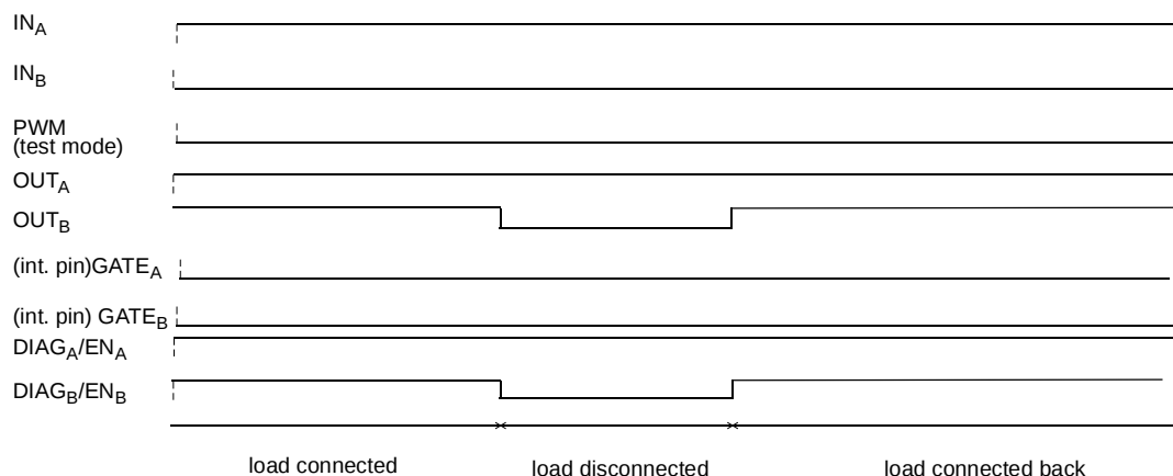
Load disconnection test (IN A =1, PWM=-2V)
